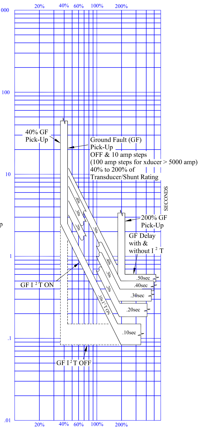
Ground Fault Time Current Curve
