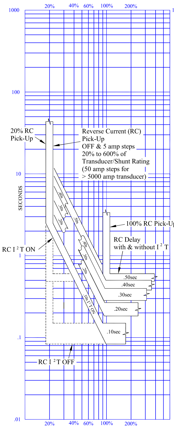
Reverse Current Time Current Curve
