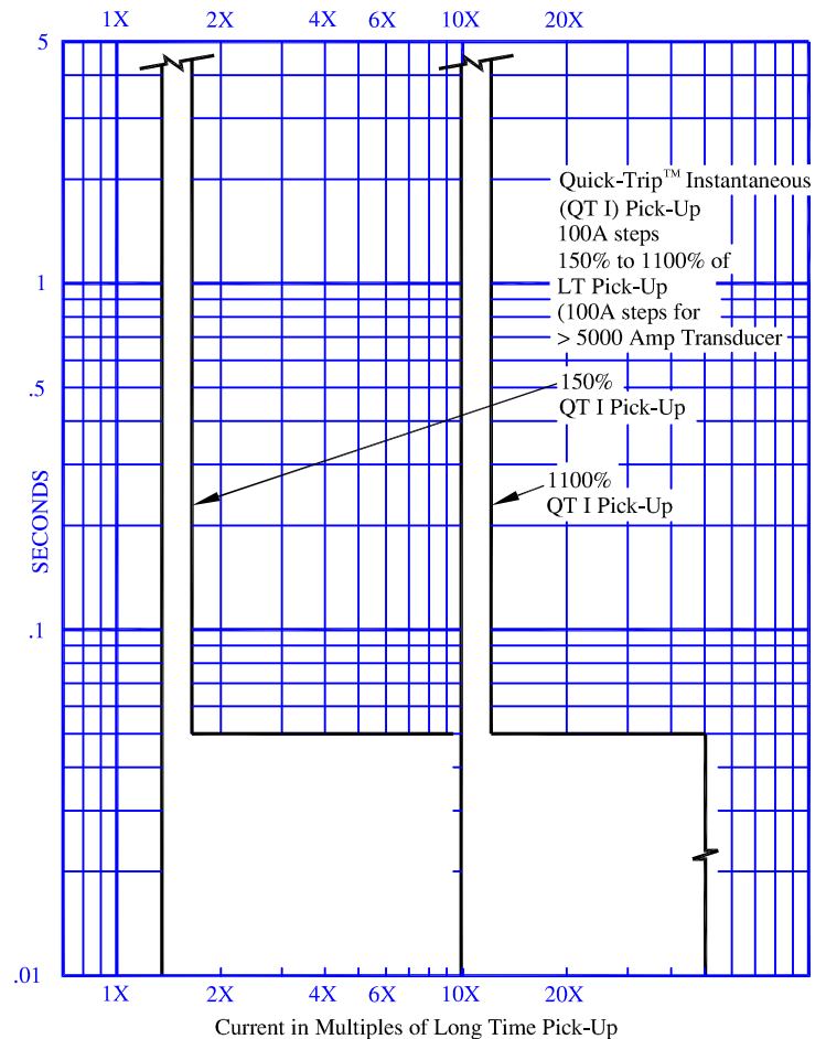
Quick-Trip™ Instantaneous Time Current Curve
