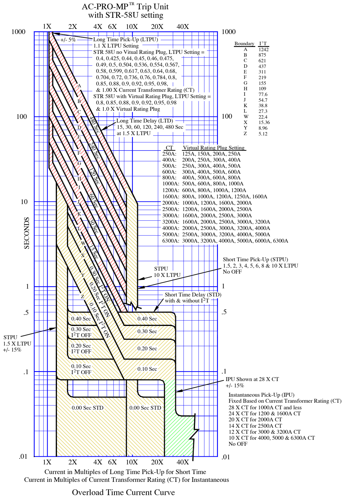
Figure 8 AC-PRO-MP TM STR-58U Time-Current-Curve
