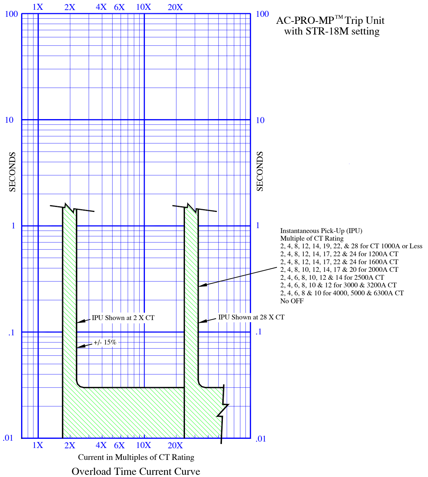
Figure 5 AC-PRO-MP™ STR-18M Time-Current-Curve
