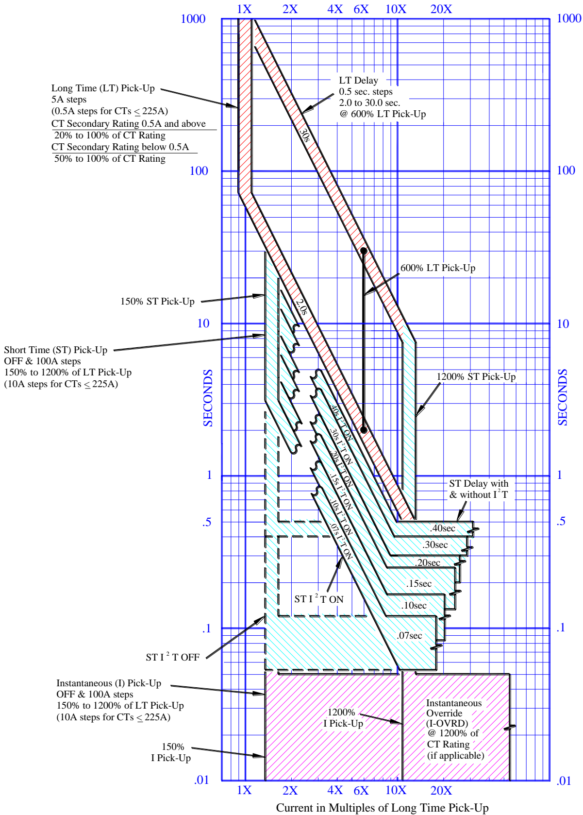
AC-PRO-II Overload Time Current Curve
