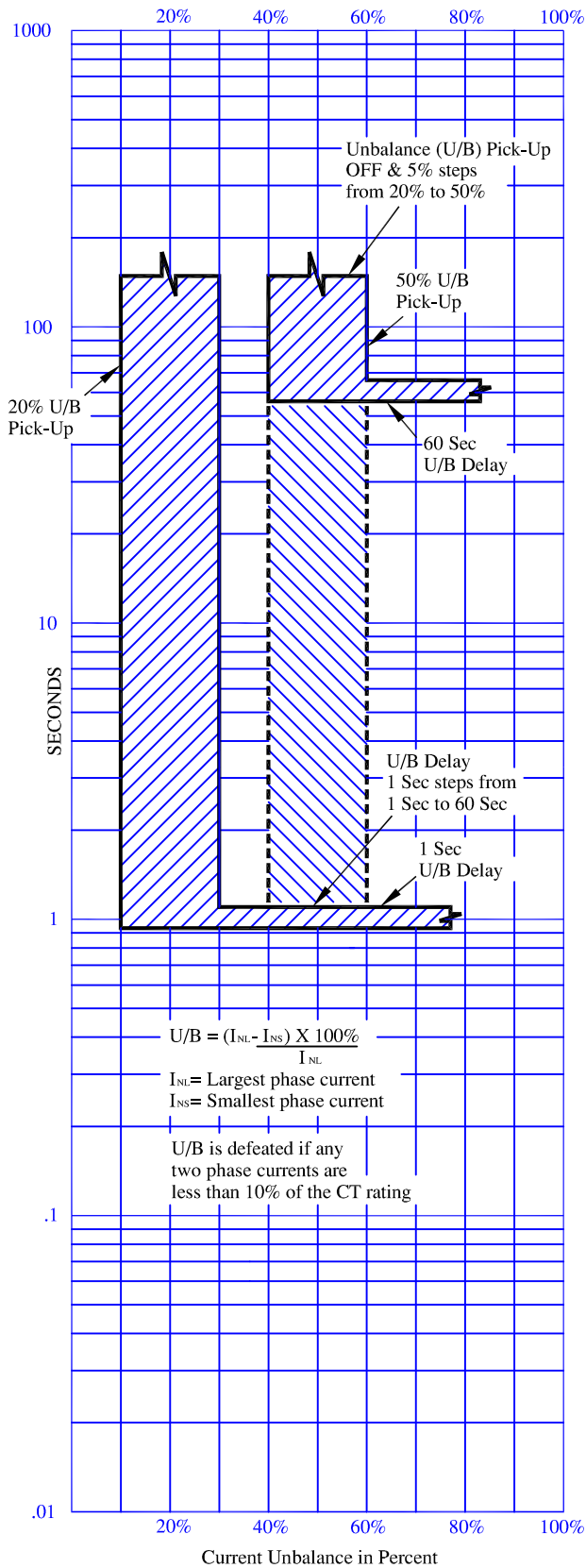
Unbalance Time Current Curve
