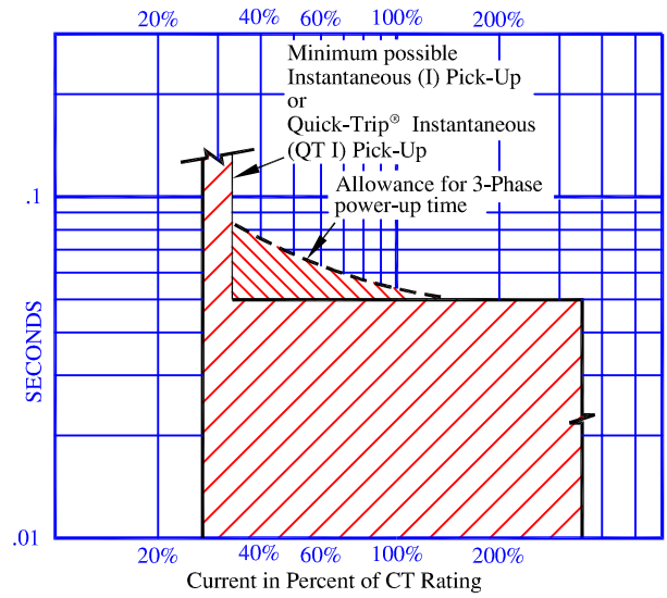
Instantaneous Allowance for 3-Phase Power-Up Time For Very Low QT-I Settings
